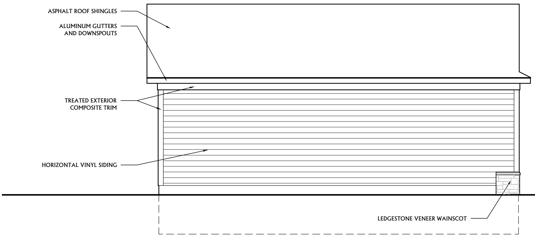
Side Elevation
