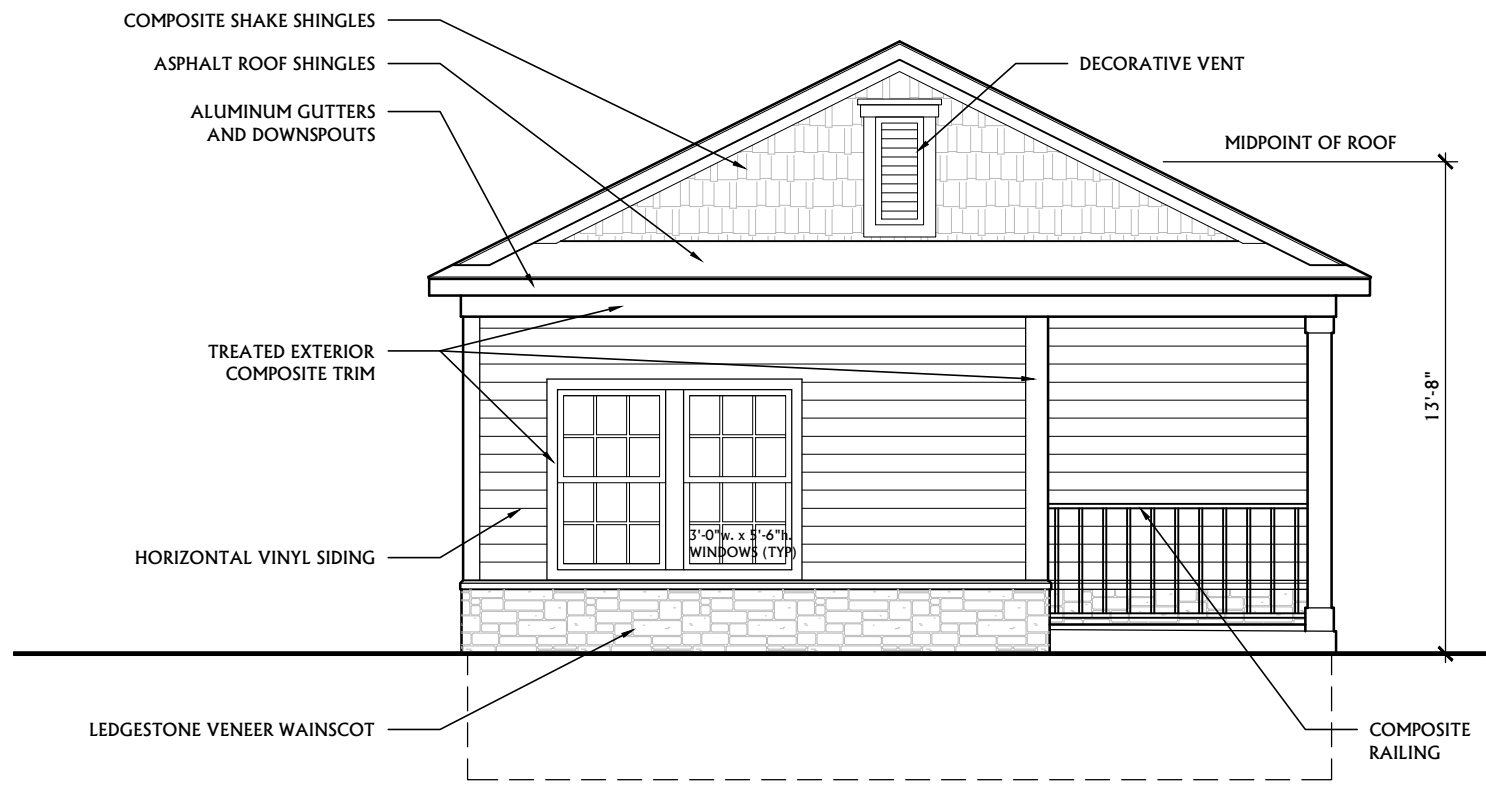
Front Elevation
